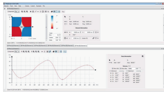
Fig. 4. Azimuthal (in-plane) angle distribution with a circle section in the middle of the magnet for Z = 2\text{mm} . In the 1D Plot, the minimum and maximum values are automatically detected and give a direct measure of the angle error of the Bxy magnetic field distribution on the circle.
