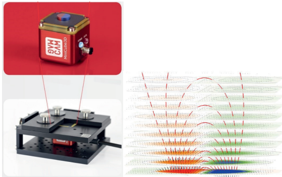
Fig. 2. 2-pole axially magnetized cylinder magnet measured with MiniCube3D magnetic field camera.
