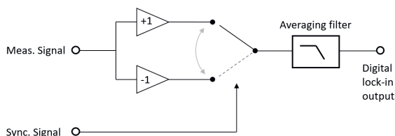
Fig. 4: Principle of the digitally implemented synchronous detector.
