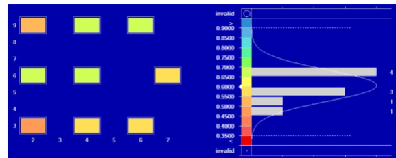
Fig. 5: Full wafer map of the integrated Ge-photodiode responsivity.
