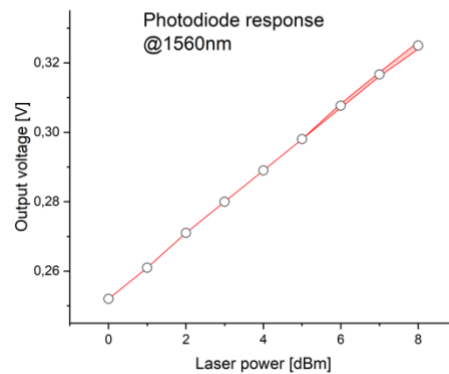
Fig. 6: Typical responsivity curve of an integrated Ge-photodiode. The responsivity is deduced from the slope of this curve. The orange line corresponds to the standard deviation.
