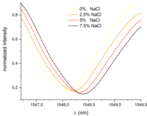
Fig. 8: Resonance peak position for different concentration of NaCl in deionized water at various weight percentages.
