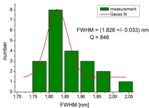
Fig. 4: Full width at half maximum (FWHM) of the partially slotted ring resonator. Each data point corresponds to one sensor chip. The data was collected on a full wafer.
