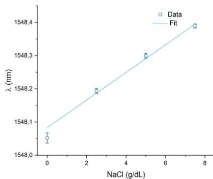
Fig. 9: Center wavelength position of each peak as a function of the NaCl concentration.
