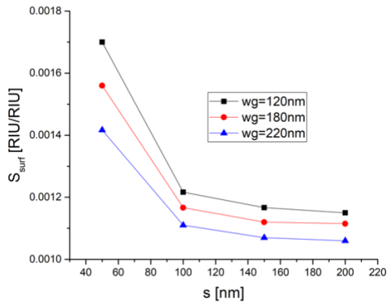
Fig. 3: Surface sensitivity as function of the slot width.
