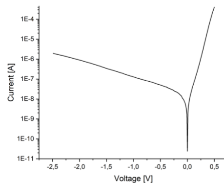
Fig. 7: Dark current of integrated Ge-photodiode.
