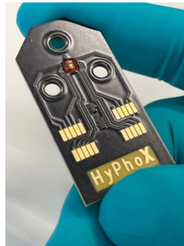
Fig. 1: Photonic biosensor chip placed on top of a PCB. Metal wire bonds connect the integrated Ge-photodiode with the PCB.
