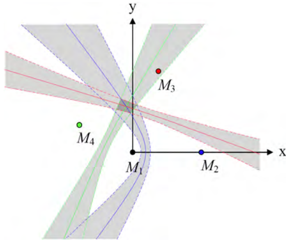
Fig. 1. The measured time difference \Delta t_{kj} between M_k and M_g yields a hyperbola (solid lines). Inequality (4) bounds a region of uncertainty where S_j can reside (grey regions), here depicted for the origin M_1 and three other receivers.
