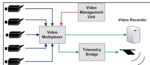
Figure 6: Camera system using video multiplexors and management unit
