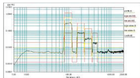
Figure 4: Random Vibration Test
