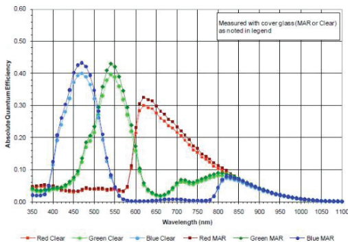
Figure 2: Spectral sensitivity of a typical CCD
