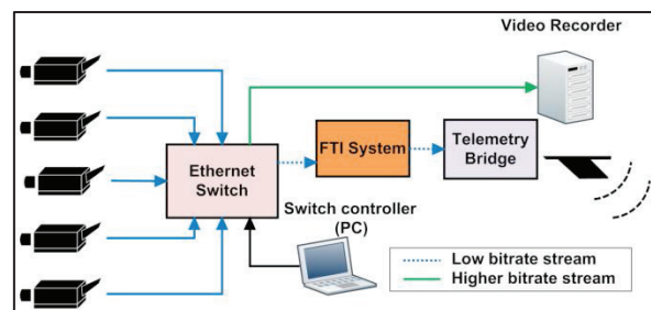
Figure 9: Dual compression on FTI cameras
