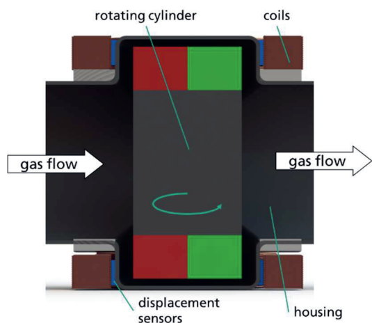
Fig. 3. Magnus sensor concept (cross-section)
