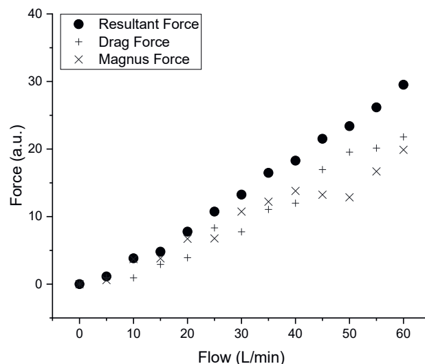
Fig. 4. Force signal for varying volume flows of 0-60 L/min at a rotational speed of 5000RPM
