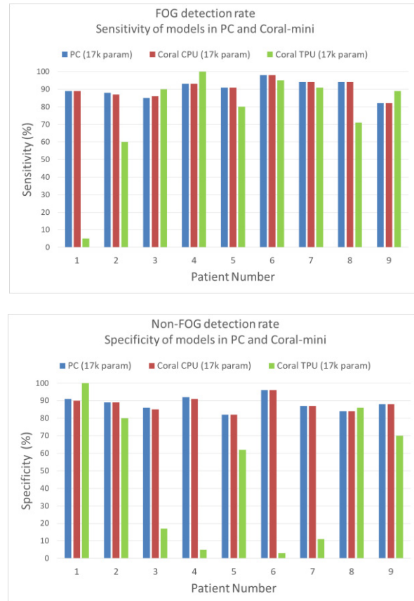
Fig. 2: Performance of the models trained on PC and the ones converted for Google Coral's CPU and TPU.
