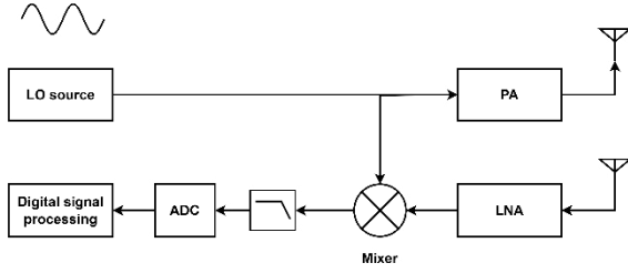
Fig. 1. A block diagram of a CW RADAR system.
