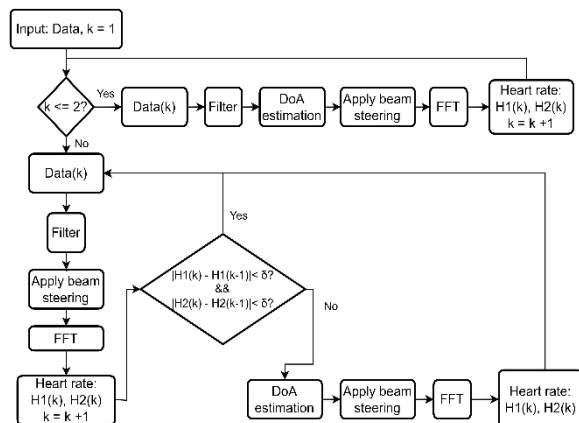
Fig. 6. Processing flow for multiple patients' heart rate monitoring.
