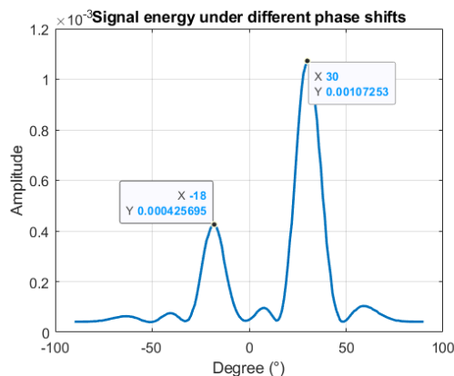
Fig. 4. Direction-of-arrival estimation via digital beam steering.
