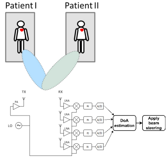
Fig. 2. Digital beam steering by adding phase shift.
