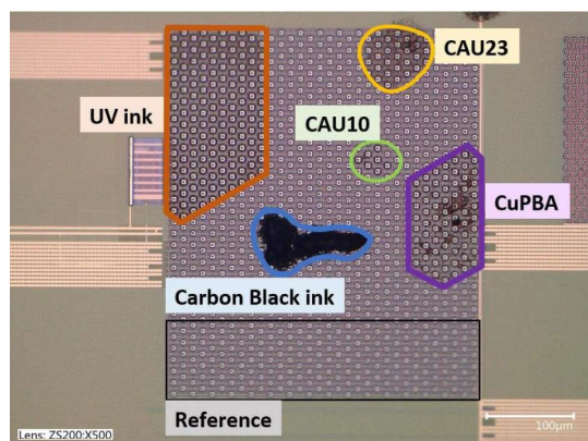
Fig. 1. Surface functionalized CMOS pixelated chip with multi-inks using an ultrasonic inkjet printer.
