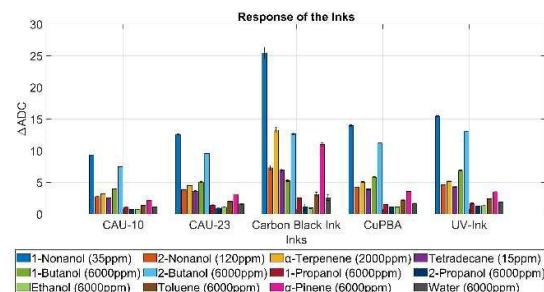
Fig. 2. E-Nose sensor's response to 11 different VOCs and humidity with 5 different inks functionalized on its surface. Tests were performed at parts-per-million (ppm) concentrations of VOCs.
