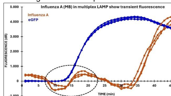
Figure 3C: Transient fluorescence observed for Influenza A (MB) in duplex reaction.
