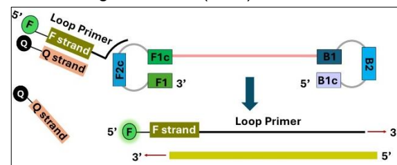
Figure 2A: Quencher strand displacement from F strand upon target recognition (working of APs).
