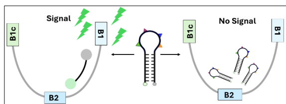
Figure 2B: Open and closed conformation of LNA incorporated molecular beacons.
