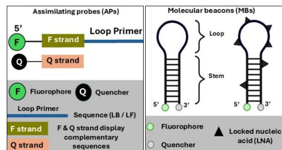
Figure 1: Left: Assimilating probe design; Right: Molecular beacon in closed conformation.
