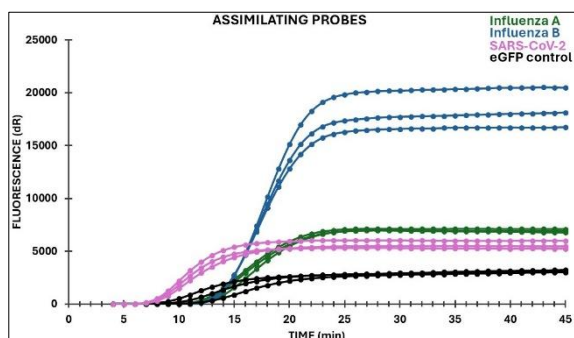
Figure 3A: Amplification plots with APs (singleplex).
