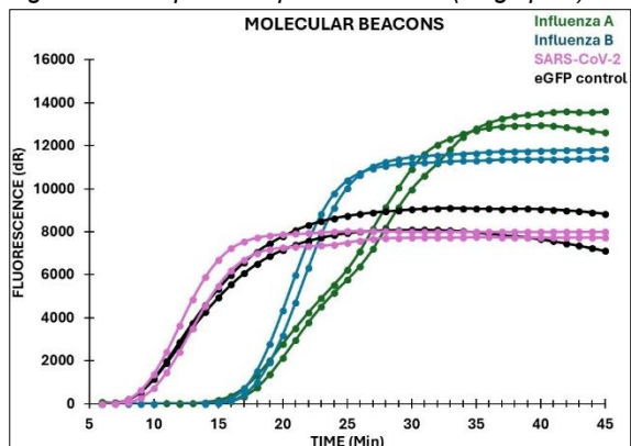
Figure 3B: Amplification plots with MBs (singleplex).
