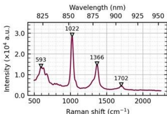
Fig. 1: Raman spectrum of an aqueous 1.0 mol/L ammonium bicarbonate solution with indicated peak positions.
