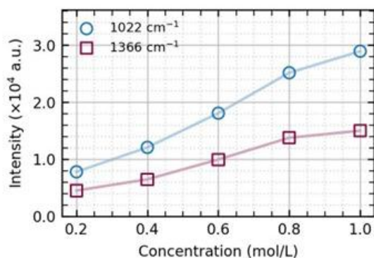
Fig. 2 Intensity of selected Raman peaks as a function of ammonium bicarbonate concentration in the range of 0.2 – 1.0 mol/L.
