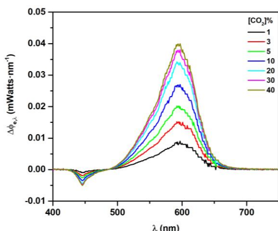
Fig. 1 CO 2 -induced change in transmitted spectral flux of the water-based MCP indicator under 2700 K white LED illumination. The main spectral change occurs around 590–600 nm, while a smaller CO 2 -dependent feature is observed near the 455 nm blue region.
