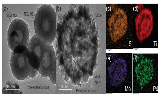
Fig. 1. (a-b) TEM images of yolk-shell ( \text{SiO}_2 - \text{TiO}_2 ) NS and \text{Pd@MoS}_2 YS ( \text{SiO}_2 - \text{TiO}_2 ) NS, corresponding EDS elemental mapping: (c) Si (d) Ti (e) Mo and (f) Pd.
