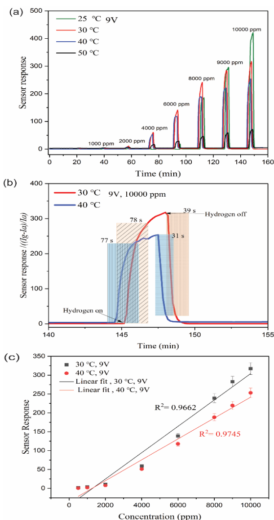
Fig. 2. Dynamic response towards hydrogen: (a) at different operating temperatures, (b) response and recovery times at 10,000 ppm, and (c) calibration curves at 30 °C and 40 °C.
