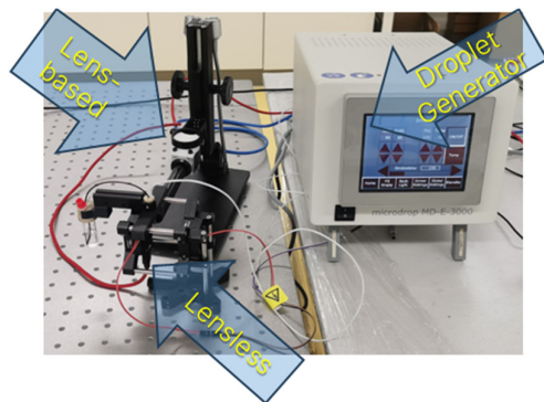
Fig. 1. The lensless microscope and lens-based imaging system were integrated to enable simultaneous image acquisition as a validation step. Furthermore, the strobe mode of the microdroplet generator was synchronized with the light sources of both the lensless microscope and the lens-based camera.
