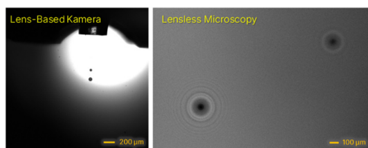
Fig. 2. The lensless microscope was capable of capturing droplet images in strobe mode. The droplet positions shifted accordingly when the frequency or strobe delay was adjusted, consistent with the observations obtained using the lens-based camera.
